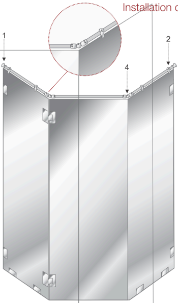
Installation of Glass Clamps
