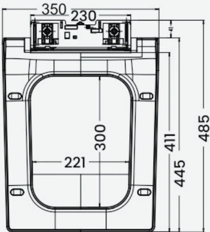
Base Plate Dimension
